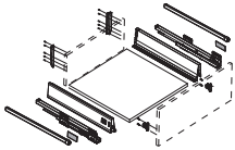
Double Wall Drawer Set Silky White Color Screw-on (Double Railing)
